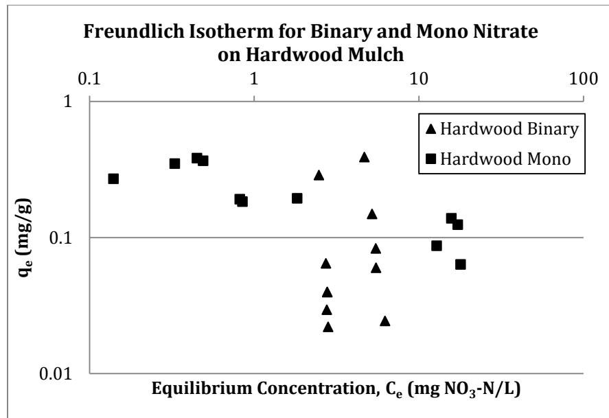
Figure L6: Freundlich adsorption isotherm for nitrate in the binary system on hardwood mulch
