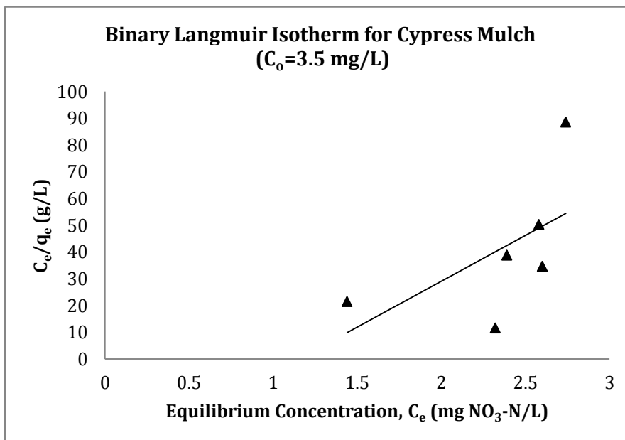
Figure K3: Langmuir adsorption isotherm for nitrate at an initial concentration of 3.5 mg \text{NO}_3\text{-N/L} in the binary system on cypress mulch
