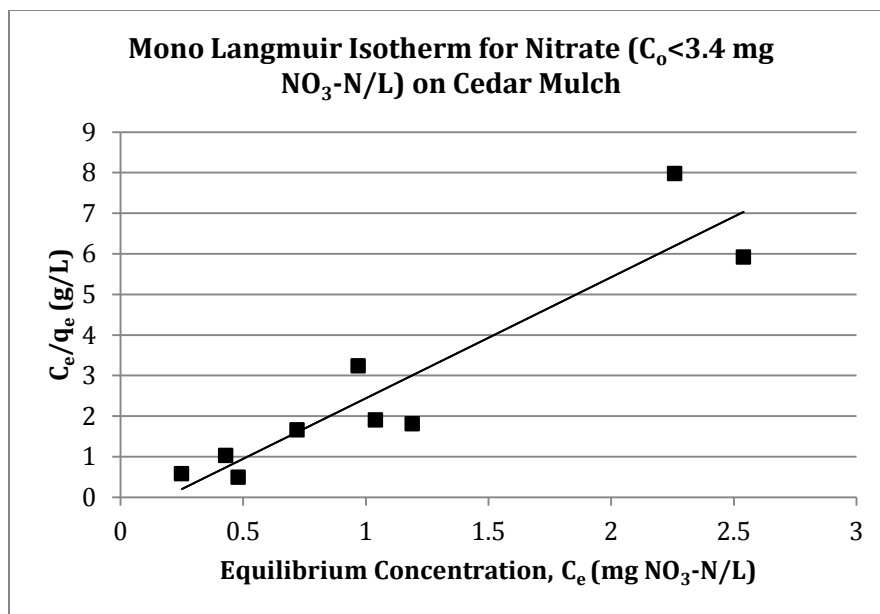
Figure E1: Langmuir adsorption isotherm for nitrate ( C_0 < 3.4 \text{ mg NO}_3\text{-N/L} ) in the mono system on cedar mulch
